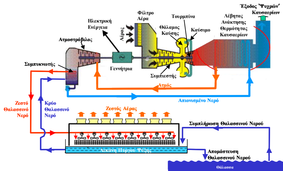
SIMPLIFIED FLOW CHART
